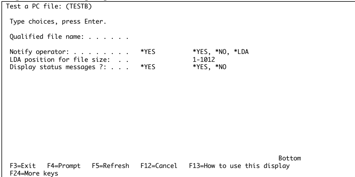
Figure 7-4 TESTB prompt screen
