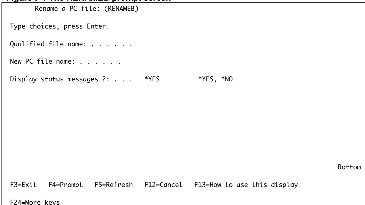
Figure 7-1 The RENAMEB prompt screen
